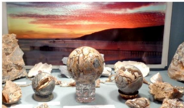
Deedeeite—Avila Beach
